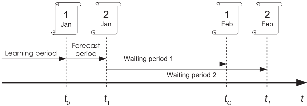
▲ Figure 1. Time line of forecasting and testing. Any model generates its forecast at t_0 using all data from the learning period. The forecast is valid for the period from t_0 to t_1 . The revised catalog for forecast generation is available after the waiting period 1 at t_C . Testing can be performed after the waiting period 2 at t_T .
