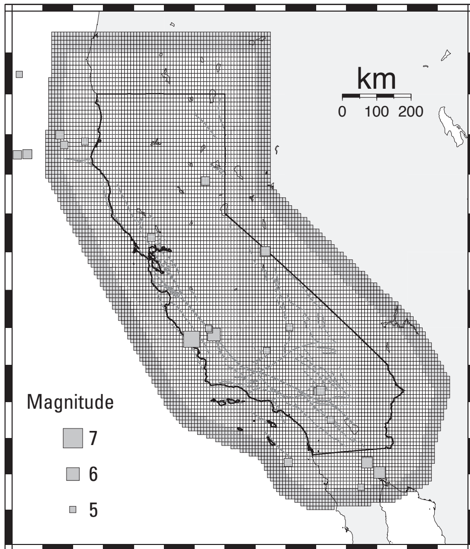
▲ Figure 2. Testing and collection area. The white squares indicate spatial cells of the testing area. The cells extending the testing area to the collection area are drawn in gray. Main faults are indicated with gray lines. The squares mark earthquakes of magnitude M \geq 5 of the ANSS catalog in the period 2000–2005.
