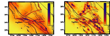
Figure 5: Examples for model expectations. (Left) Nodewise sum of expectations of a grid-based model derived from the USGS 1996 model [Frankel et al., 1996]. (Right) Nodewise sum of expectations of the model from [Helmstetter et al., submitted].
