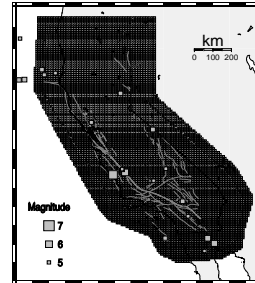
Figure 4: Testing and data collection bins. Testing bins are plotted as white patches. The collection areas additionally contains the bins plotted as dark gray patches. Light gray patches indicate events of magnitude M \geq 5 of the last 5 years.
