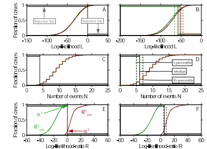
Figure 6: Examples for results of a 5-years test comparing the models shown in Figure 5. Green lines indicate CDFs of simulations of the model by [Frankel et al., 1996], red lines of the model by [Helmstetter et al., submitted], respectively. The vertical lines indicate the observed values (including bootstrap over uncertainties). (Left column) Results from the L-Test, N-Test, and R-Test using an undeclustered catalog. (Right column) Results from the L-Test, N-Test, and R-Test using a catalog with independence probabilities.
