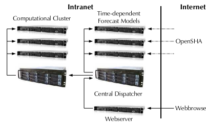
Figure 3: Schema of the computer setup for the Testing Center. The Central Dispatcher is conducting the tests and storing the results. Each time-dependent model runs on a model computer, additionally accessible from the internet via OpenSHA. All results will be presented on the webserver.
